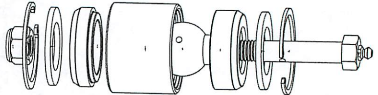
KU70088 2.5" Poly Flex Joint Upgrade kit
